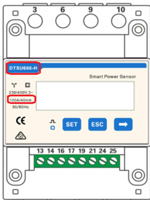
Figure 2-10 DTSU666-H
