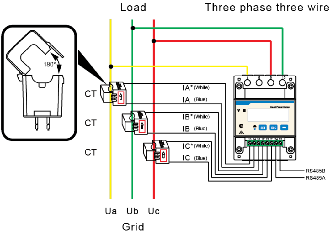
Figure 4-2 Three-phase three-wire (supported model: DTSU666-H 250 A/50 mA)
