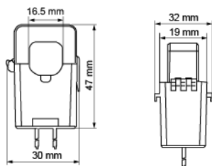
Figure 2-8 100 A CT dimensions
