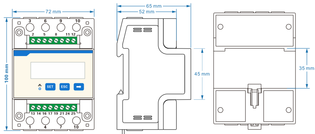
Figure 2-7 Product dimensions (Smart Power Sensor)
