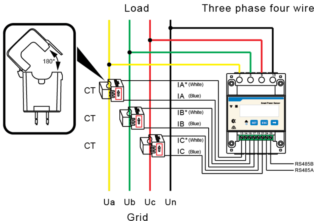
Figure 4-1 Three-phase four-wire (supported model: DTSU666-H or DTSU666-H 250 A/50 mA)
