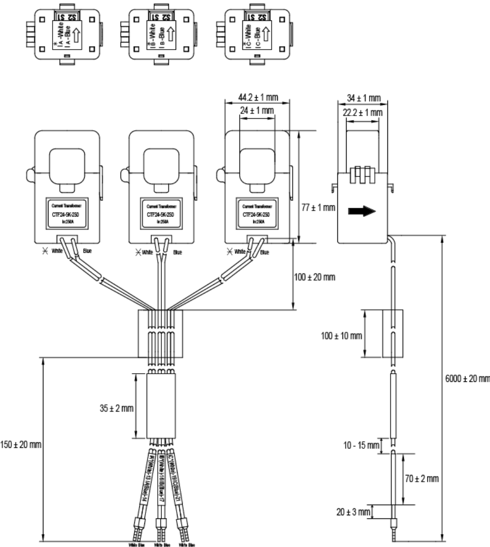
Figure 5-3 CT structure of the DTSU666-H 250 A/50 mA
