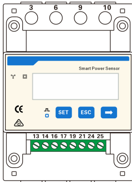
Figure 2-1 DTSU666-H or DTSU666-H 250 A/50 mA
