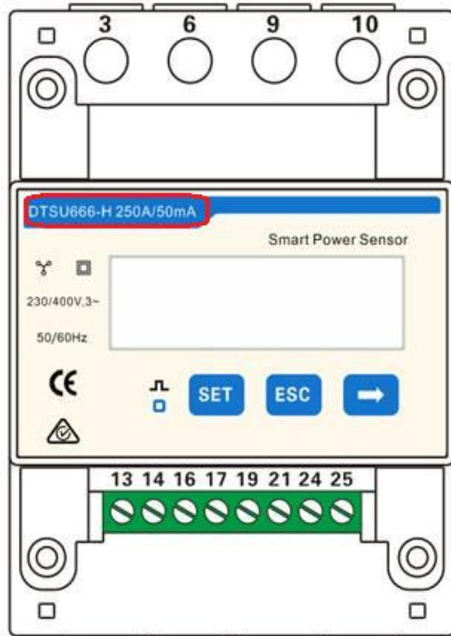
Figure 2-11 DTSU666-H 250 A/50 mA
