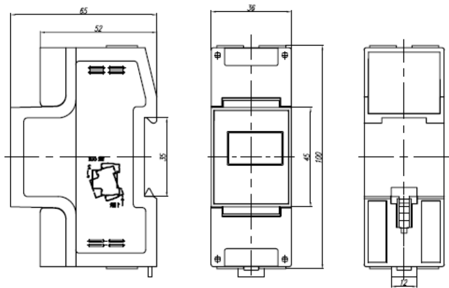
Figure 2-7 Product dimensions
